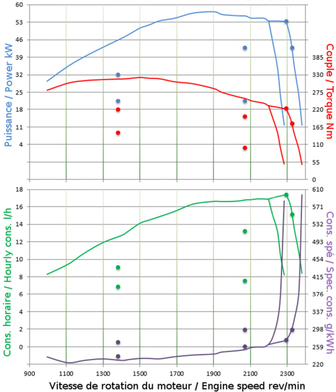
NEW HOLLAND T 4.85 4WD
