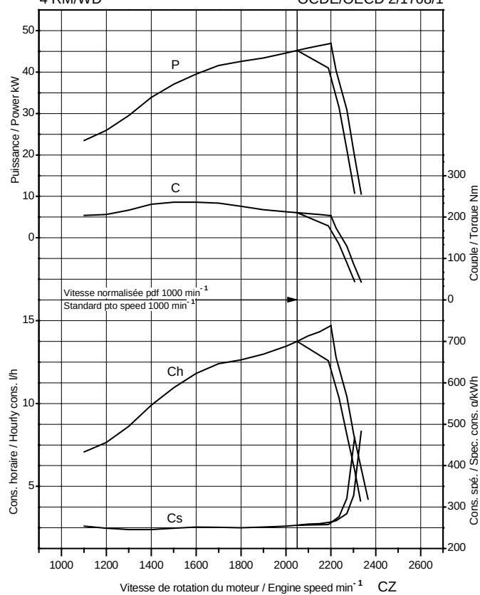
Zetor 6341 Super (40 km/h)
