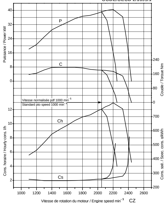
Zetor 4341 Super (40 km/h)
